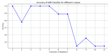
Fig. 6. Accuracy trend for varying k values.
