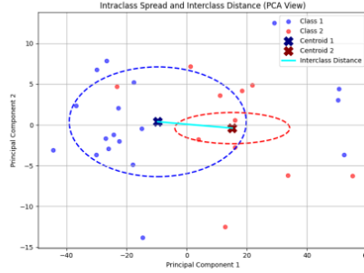
Fig. 4. PCA visualization depicting class clusters and centroid separation.
