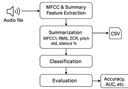
Fig. 1. Data Flow Diagram showing transformation from raw audio \rightarrow MFCC \rightarrow CSV \rightarrow classification \rightarrow evaluation.
