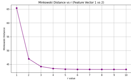
Fig. 5. Minkowski Distances vs r
